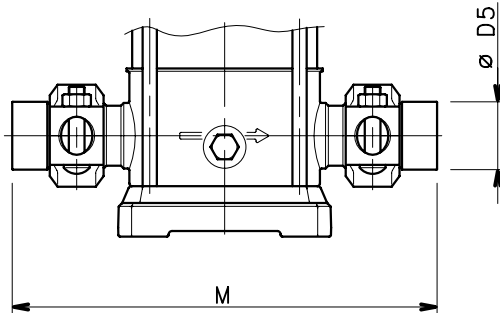
WELD-ON SLEEVES
