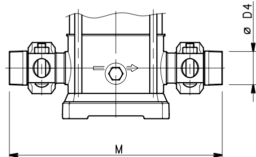
THREADED SLEEVES
